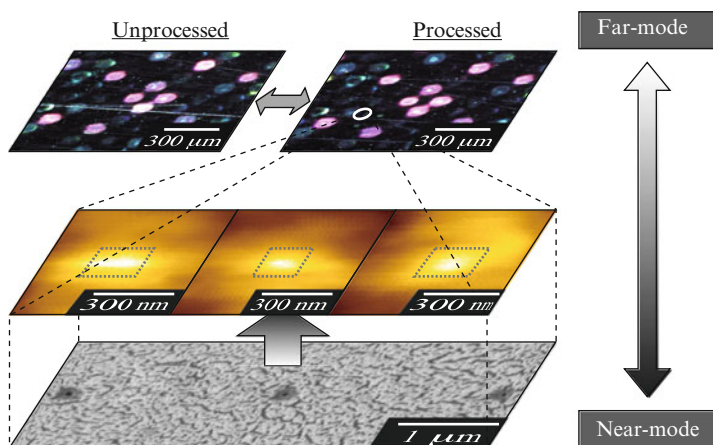
Fig. 2.13 (Upper) Observed CCD image of sample hologram. (Middle) Magnified image of processed hologram and (Lower) corresponding optical response observed with an NOM
