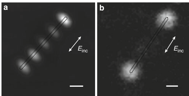
Fig. 4.15 Two-photon excitation images of single gold nanorods. (a) diameter 20 nm, length 540 nm, (b) diameter 21 nm, length 565 nm. The images are taken at 780 nm excitation. Dotted lines: approximate shape of the nanorod. Scale bars: 100 nm
