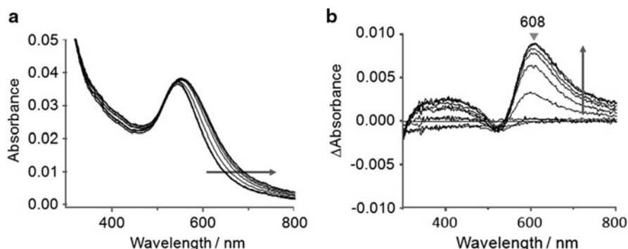
Fig. 5.14 (a) Absorption spectra taken during titration of Phenaz-TMA/AuNPs with λ-DNA and (b) their difference spectra. Here 0, 5, 10, 15, 20, 25, 30, 35, 40, 45, and 50 \mu\text{L} of DNA ( 4.5 \text{ ng } \mu\text{L}^{-1} ) solutions were added to 3 mL of Phenaz-TMA/AuNP ( 143 \mu\text{g mL}^{-1} ) aqueous solution. Reprinted with permission from [80]. Copyright (2010) by the Japan Society for Analytical Chemistry
