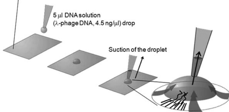
Fig. 5.5 Procedure of DNA stretching and alignment on surfaces
