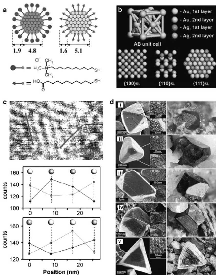
Fig. 6.16 (a) Scheme and average dimensions (in nanometer) of AuMUA and AgTMA nanoparticles used as the model system. Particle compositions are Au 4100 L 380 (where L is MUA) and Ag 3400 L 340 (where L is TMA); (b) Scheme of an AB unit cell and the projections of {100}SL, {110}SL, {111}SL planes. (c) Compositional analysis of the NP crystal faces. Upper: STEM image of a hexagonal {111} face, lower: the EDS analysis in STEM mode. (d) Different morphologies of the AuMUA-AgTMA crystals (left column) and their macroscopic sphalerite (SL) (i–iv) and diamond (v) counterparts (right column). (i) Octahedron; insets show {111}SL and {100}SL faces. (ii) Cut tetrahedron; insets show {111}SL and {100}SL faces from cut top and from cut edge, respectively. (iii) Octahedron with two triangular faces cut; inset shows the {111}SL face. (iv) Twinned octahedron; insets magnify {111}SL faces at the location of twinning and the {100}SL face of a broken neighboring crystal. (v) Truncated tetrahedron; inset shows top view of the {111}SL face [67]
