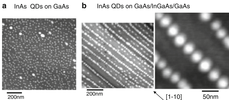
Fig. 3.38 AFM images of InAs QDs, grown, respectively, on GaAs buffer layer (a) and on GaAs/InGaAs/GaAs buffer layer (b). InAs QD chains were aligned along [1\bar{1}0] direction on the GaAs/InGaAs/GaAs (b)
