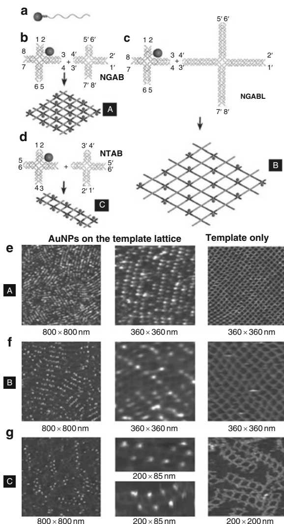
Fig. 6.24 Schematic representations of the DNA-templated assembly of periodical AuNP nanoarrays. (a) 1:1 conjugate of a Au NP (ball) with a thiolated DNA strand (curved line). (b) AuNP on an NGAB lattice (A). The DNA strands self-assemble into the cross-shaped A (blue) and B (orange) tiles with sticky ends so that 1 is complemented with 1', 2 with 2', and so forth. The central strand on A tile carries the AuNP into the self-assembled 2D nanogrid. (c) A AuNP on an NGABL lattice (B). The A tile remains the same as in (b), and the four arms of the B tiles are each elongated by four DNA helical turns, thus the 2D arrays assembled have a larger cavity. (d) A AuNP on an NTAB lattice (C). They self-assemble into 1D nanotracks by modifying the sticky ends of the A and B tiles. Note: all the A tiles share the same central strand that carries the AuNP. AFM images show the patterning of AuNPs on the self-assembled DNA nanostructures. (e) AuNPs on NGAB lattices (A). (f) AuNPs on NGABL lattices (B). (g) AuNPs on NTAB lattices (C) [103, 105]
