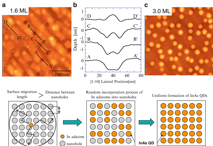
Fig. 3.16 AFM images of second InAs islands with 1.6 ML (a, b) and 3.0 ML (c), which were grown on GaAs nanoholes. Fig. 3.16b shows line profiles at various positions of the nanoholes in (a). Insert of schematic diagram indicates selective formation process of second InAs QDs on nanoholes. Uniform first InAs QDs were embedded under nanoholes
