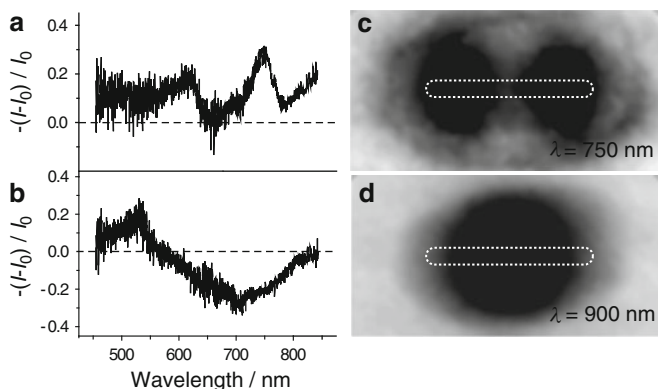
Fig. 4.11 (a,b) Polarized near-field transmission spectrum of a gold nanorod (diameter 30 nm, length 300 nm); polarization parallel (a) and across (b) to the long axis of the nanorod. (c), (d) Polarized near-field transmission images obtained at 750 and 900 nm, respectively. Polarization is parallel to the long axis of the nanorod. Dotted lines: approximate shape of the nanorod
