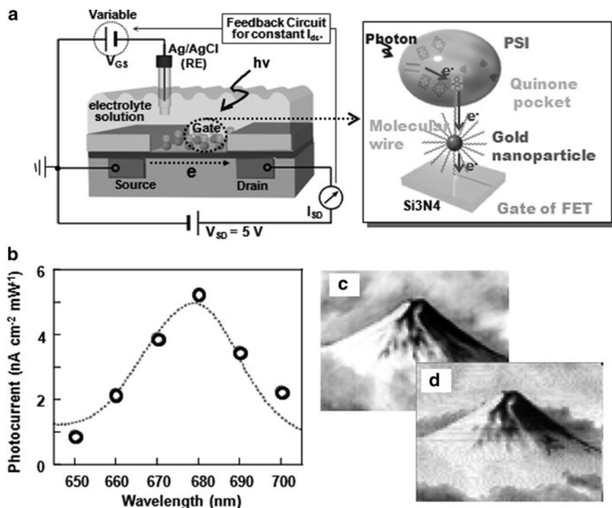
Fig. 6.32 (a) Schematic illustration of the FET module with the gate modified with nanoparticle-reconstituted PSI molecules (left). The concept of photosensor composed of nanoparticle-reconstituted PSI (right). A photon is converted to an electron and transferred to a gold nanoparticle. (b) A photocurrent action spectrum upon nanoparticle-reconstituted PSI molecules immobilized gold electrode ( \circ ). Dotted line is an absorption spectrum of PSI molecules. (c) An input image and (d) the out put image obtained with the FET system (a) [144, 145]
