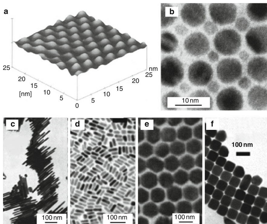
Fig. 6.9 (a) STM image of self-assembled superlattice of 3.5 nm gold particles on an HOPG substrate. The particles are stabilized by hexanethiol [43]. (b) TEM micrograph of a section of an AB (NaCl-type) superlattice of silver nanoparticles stabilized by decanethiol having a bimodal size distribution [47]. Self-assembly patterns formed by various shapes and sizes of gold nanoparticles, as visualized by TEM. (c) Ribbon structure formed from nanorods of high aspect ratios ( >5 ); (d) globally isotropic but locally ordered arrangement of nanorods of low aspect ratios; gold nanocrystals with hexagonal profiles (e) and cubic profiles (f)
