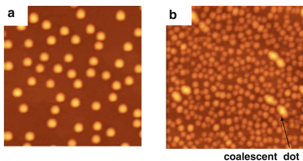
Fig. 3.23 AFM images of low-density InAs QDs (a) and high-density InAs QDs (b). (a): growth temperature of 500^{\circ}\text{C} , growth rate of 0.035 \text{ ML s}^{-1} , arsenic pressure of 3 \times 10^{-6} \text{ Torr} , (b): 480^{\circ}\text{C} , 0.070 \text{ ML s}^{-1} , 6 \times 10^{-6} \text{ Torr}
