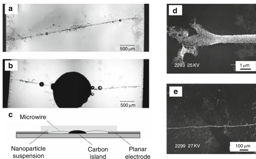
Fig. 6.21 (a) A composite optical micrograph of a gold microwire spanning a 5-mm gap between planar gold electrodes. (b) Two wires that have connected to opposite sides of a conductive carbon island deposited in the middle of the gap, and (c) schematics of the above configuration. (d) SEM image of the end of a growing microwire showing the structure in the growth area and uniform cylindrical porous body. (e) SEM image of a long and thin microwire [89]
