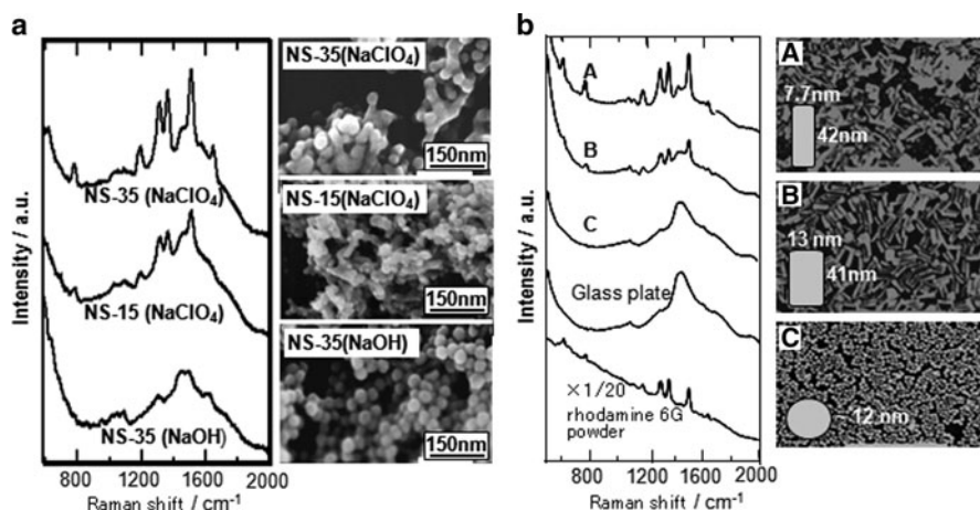
Fig. 6.29 (a) (left) Nonresonance Raman scattering spectra of rhodamine 6G (R6G) on the gold nanoparticle sample plates and (right) the SEM images of the surface of the corresponding sample plates. NS-35( \text{NaClO}_4 ): Plate prepared with 35-nm sized gold nanoparticles deposited by addition of an aqueous \text{NaClO}_4 (3M) solution. NS-15( \text{NaClO}_4 ): Plate prepared with 15-nm sized gold nanoparticles deposited by addition of an aqueous \text{NaClO}_4 (3M) solution. NS-35( \text{NaCl} ): Plate prepared with 35-nm sized gold nanoparticles deposited by addition of an aqueous \text{NaCl} (3M) solution. (b) (left) Nonresonance Raman scattering spectra of R6G on the gold nanoparticle or nanorod sample plates and (right) the SEM images of the surface of the corresponding sample plates. (A) Plate prepared with gold nanorods with the diameter of 7.7 nm and the length of 42 nm. (B) Plate prepared with gold nanorods with the diameter of 13 nm and the length of 41 nm. (C) Plate prepared with gold nanoparticles with the diameter of 12 nm [136, 137]
