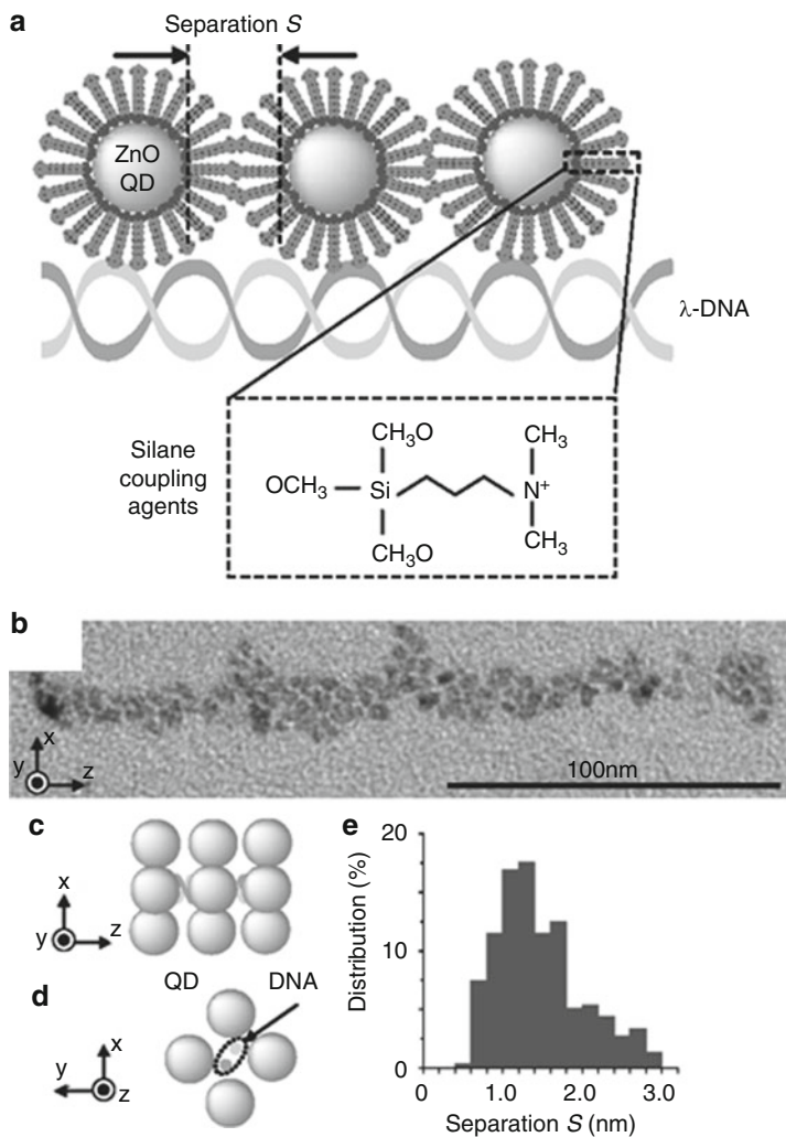
Fig. 6.19 (a) Schematic illustration of cationic ZnO quantum dots (QDs) alignment along the \lambda DNA. S : separation between QDs. (b) TEM image of aligned ZnO QDs on DNA. (c) and (d) Schematic illustrations of the QD alignment along the DNA. (e) Distribution of the separation lengths between QDs ( S ) [91]
